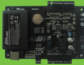
C3-100-PRO
